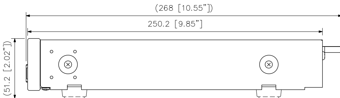
Side View
